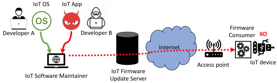
Fig. 1. A SUIT update scenario (inspired by [29]) where a developer is able to introduce a malicious app in the update pipeline.
