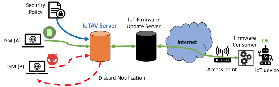
Fig. 2. SUI Update process with IoTAV. The IoTAV Server ensures that the IoT app bundled in the software update is compliant with the security policy.
