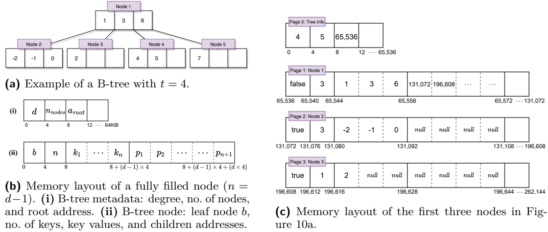
Figure 10 Memory layout of a simple B-tree.
