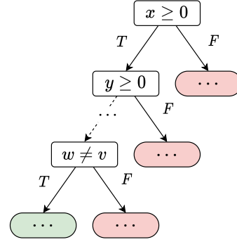
(b) Execution tree for the example in Listing 8a, where the red nodes imply a restart in WASP.
