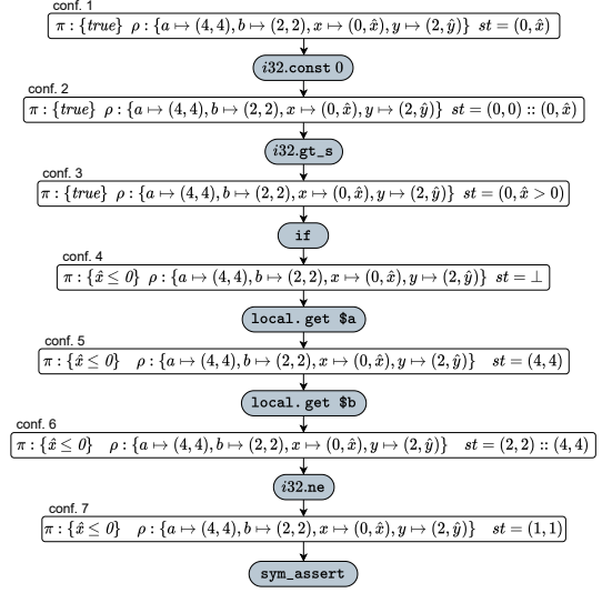
(b) Concolic execution flow diagram for the program in Listing 2a, executing the sequence of instructions indicated in lines: 4-6, and 21-24.
