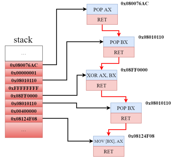
Fig. 2: An example of a ROP attack.
