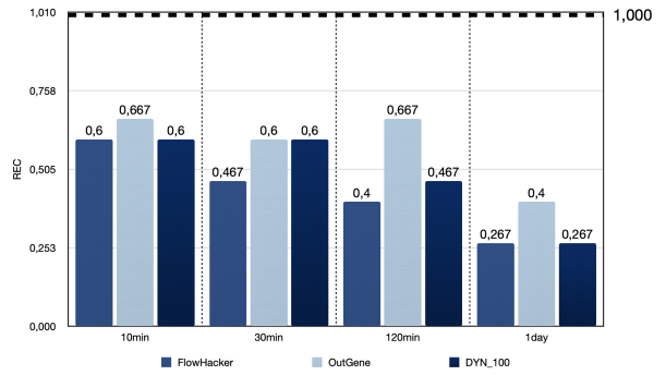
Fig. 4. REC comparison in OutGene, FlowHacker and DynIDS for the artificial dataset
