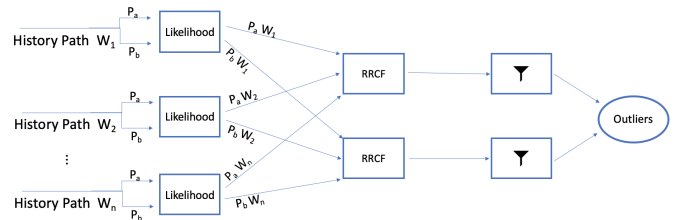
Fig. 2. Outlier detection Framework
