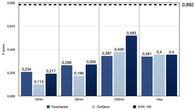
Fig. 5. F-score comparison in OutGene, FlowHacker and DynIDS for the artificial dataset
