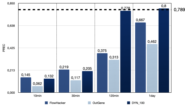
Fig. 3. PREC comparison in OutGene, FlowHacker and DynIDS for the artificial dataset
